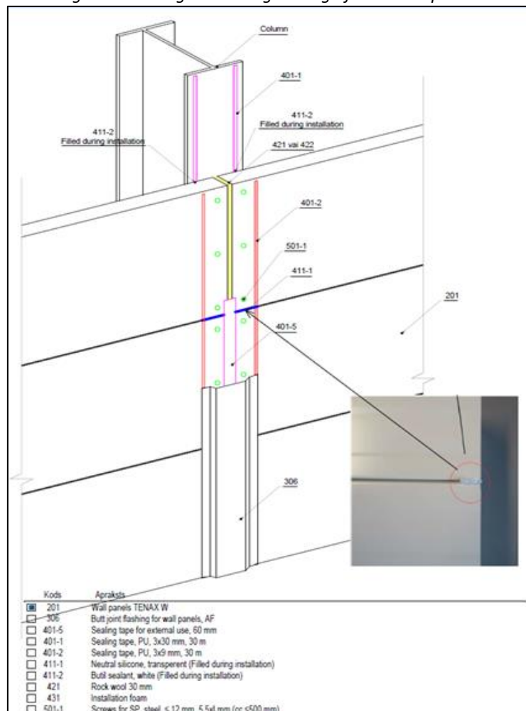
Figure 7. Sealing and strengthening of sandwich panels
