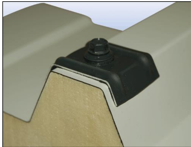
Figure 13. Fastenings for sandwich panels Tenax TR
