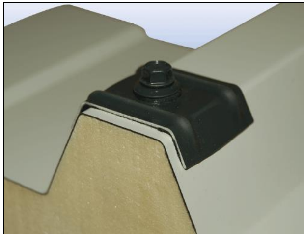
Figure 12. Fastenings for sandwich panels Tenax TR
