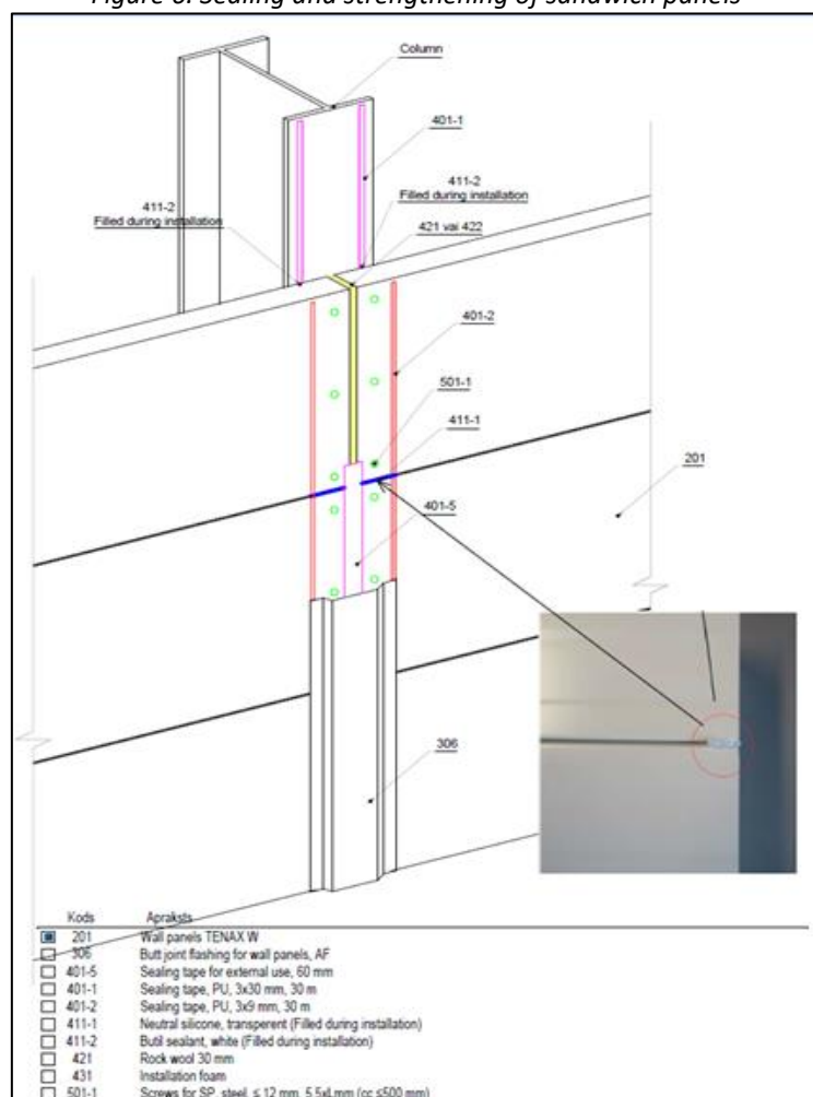
Figure 6. Sealing and strengthening of sandwich panels
