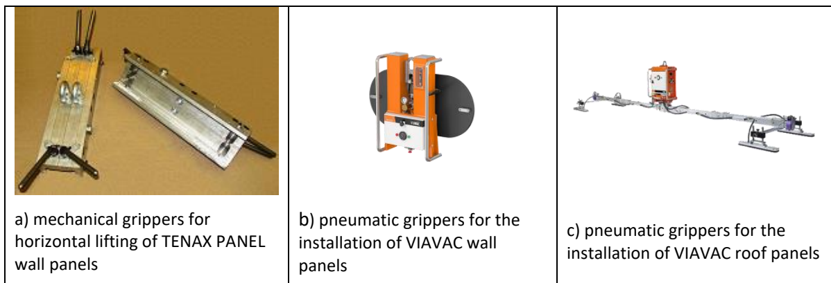
Figure3. Examples of gripping devices
