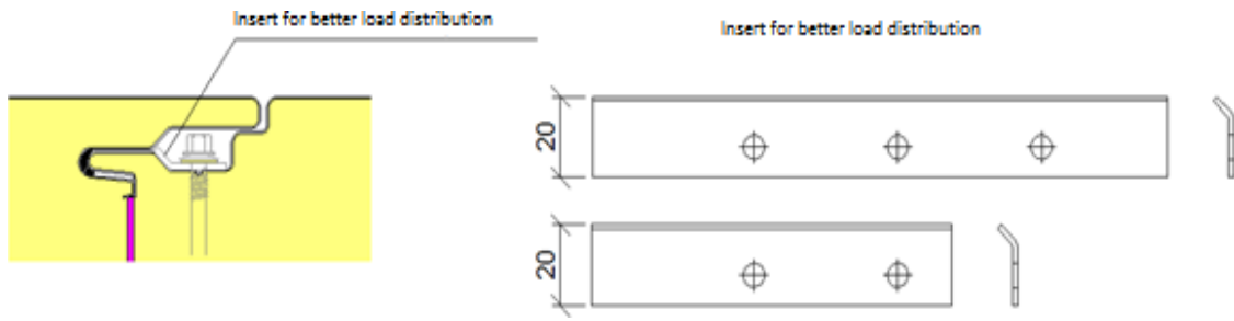
Figure 8. Tightening of screws on TENAX W sandwich panels with a hidden key (side joint H
