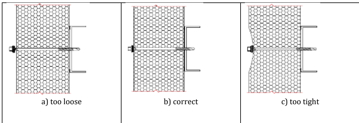
Figure 7. Tightening of screws on TENAX W sandwich panels with a standard key (side joint S or T)
